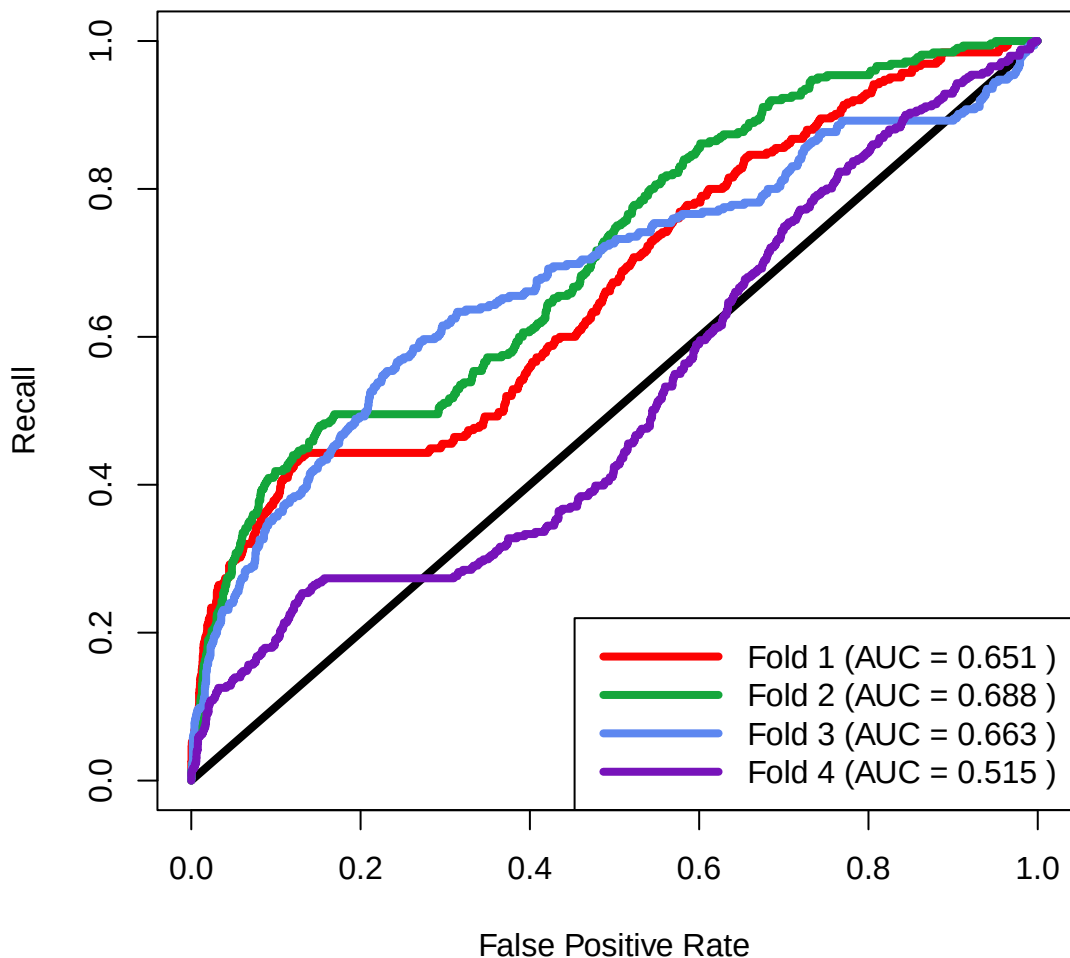
SPELL Network 430 Dataset: 430x20x10x1 Batch 50 Validation
